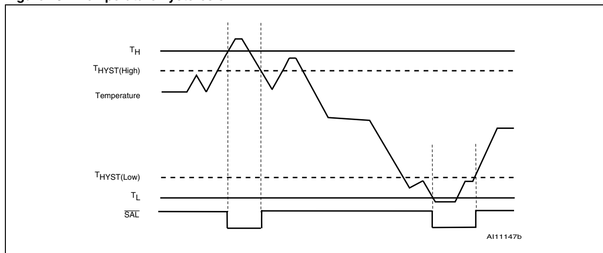
Figure 28. Temperature hysteresis
